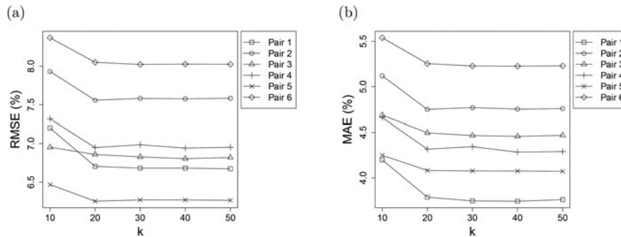
Figure A1. Prediction performance varying with different values of k s: (a) in terms of RMSE and (b) in terms of MAE.
