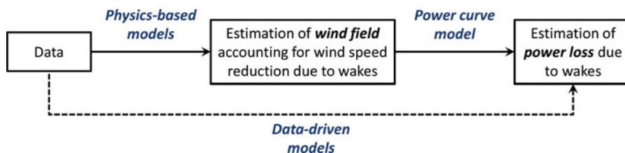
Figure 2. Wake power loss estimation procedures.
