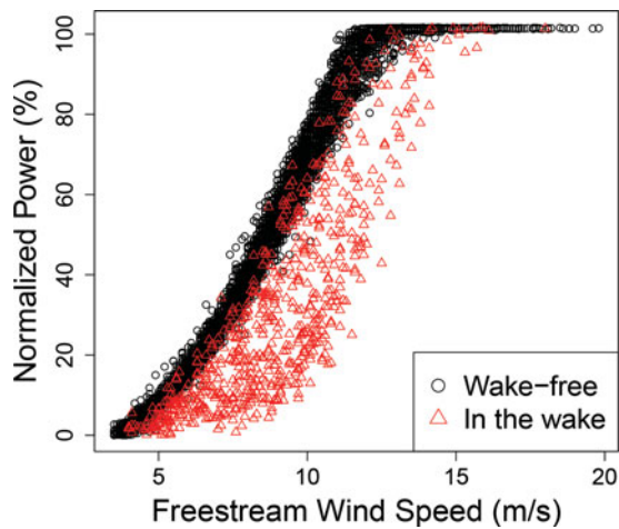
Figure 1. Power output in the wake versus that under a free-stream condition. Free-stream wind speed refers to wind speed measurements not affected by another turbine. Due to confidentiality concerns, power output is denoted throughout this article by a percentage value normalized to its maximum.
