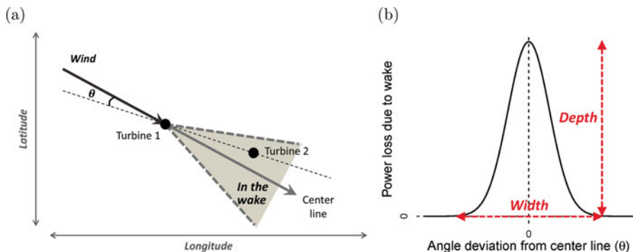
Figure 3. Characteristics of wind turbine wake and its effect: (a) wake region and \theta and (b) wake depth and wake width. Wake power loss is expected to be a function of \theta .
