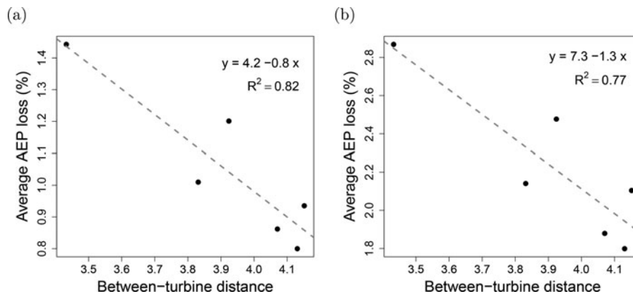
Figure 9. Relation between AEP losses and turbine spacing: (a) for the capacity factor AEP loss and (b) for the traditional AEP loss. The between-turbine distance is expressed as a multiple of the rotor diameter.
